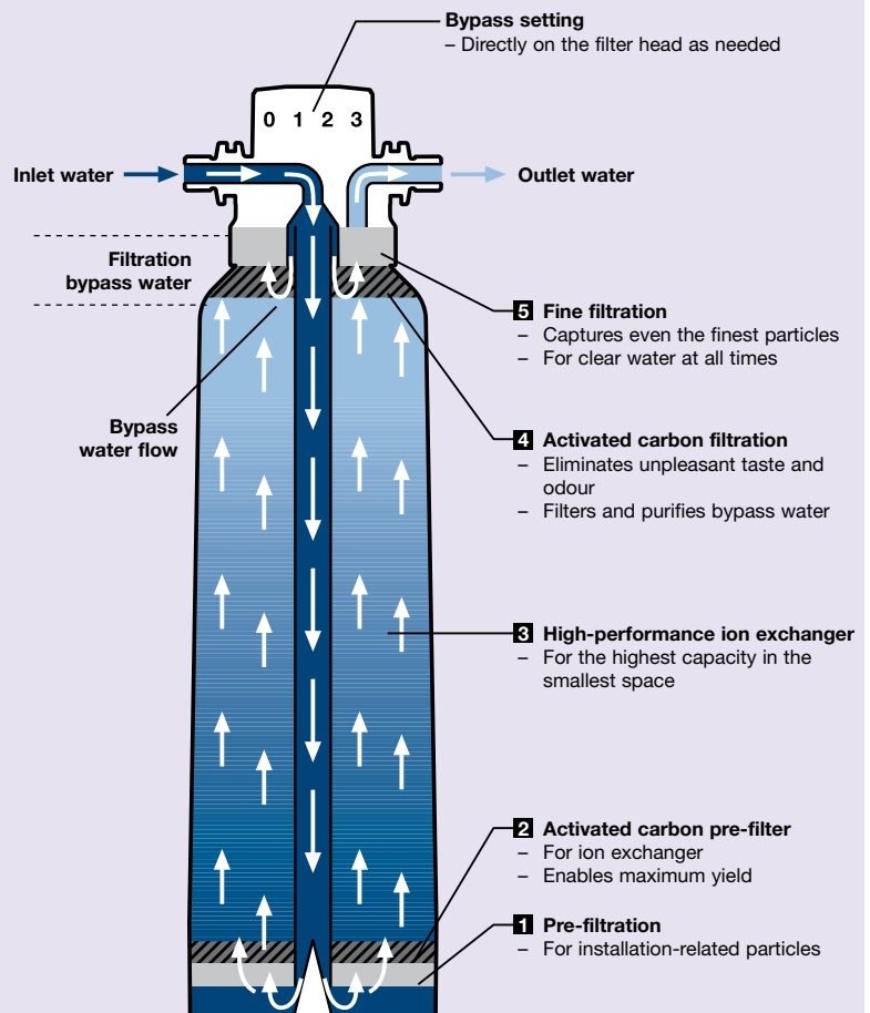
Configuration of a BWT bestprotect filter cartridge with 5-way filtration
